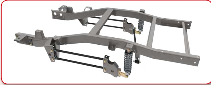
Under-Bed Coil-Over Rear Frame Clip System
